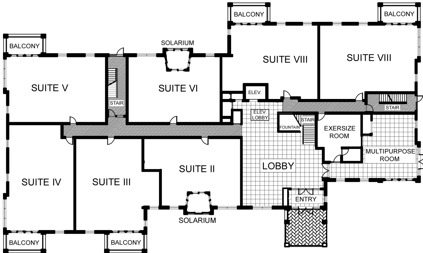
GROUND FLOOR KEY PLAN AVONLEE CONDOMINIUM, PERTH, ONTARIO
